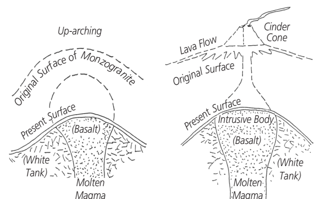
MALAPAI HILL CROSS-SECTION TWO POSSIBLE INTERPRETATIONS
