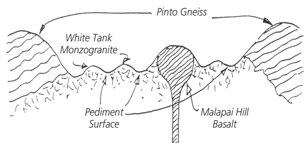
CROSS-SECTION OF QUEEN VALLEY
