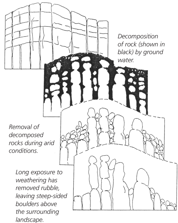
Vertical section with varied spacing of joints some 20 million years ago.
